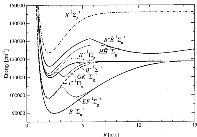
Figure 1. Potential curves for the B^1\Sigma_u^+ , B''\bar{B}^1\Sigma_u^+ , C^1\Pi_u , EF^1\Sigma_g^+ , GK^1\Sigma_g^+ , H'^1\Pi_g , HH\bar{H}^1\Sigma_g^+ and B^1\Sigma_g^+ states in hydrogen. The thick curves refer to ungerade states and the thin curves to gerade states. The \Sigma states are depicted with full curves; \Pi states with broken curves. The potential curve for the ground state of HD^+ is depicted as a dot-dashed curve.
