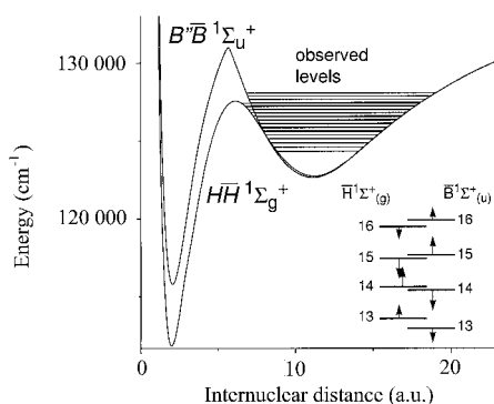
Figure 3. BO potential curves of the HH^1\Sigma_g^+ and B''B^1\Sigma_u^+ states taken from [12] and [13] respectively. Vibrational spacings in the B outer well are larger than those in H , giving rise to a crossing near v = 14 . In the inset it is shown how the levels are shifted around v = 14 .
